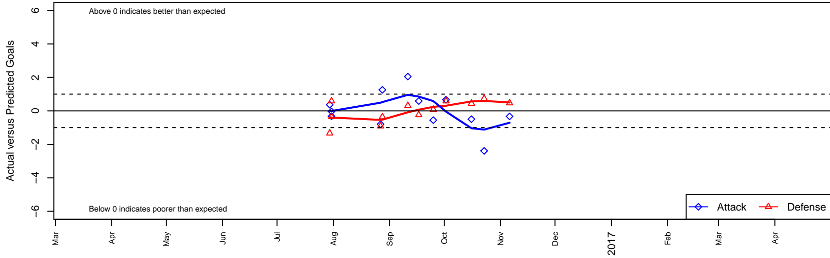
Santa Clara Sporting Green G01 Dots are actual minus expected GF (blue circles) and GA (red triangles). Blue line is smoothed change in attack strength. Red is smoothed change in defense strength.
